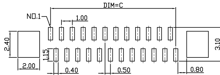
RECOMMENDED P.C.B LAYOUT NEGATIVE-NEEDLE CIRCUIT BOARD
